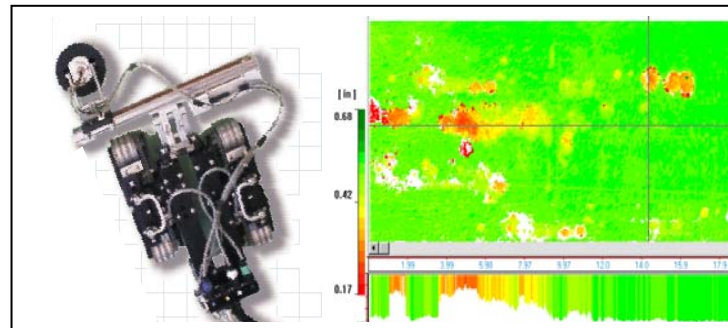
Computerized Crawler / Corrosion Map
